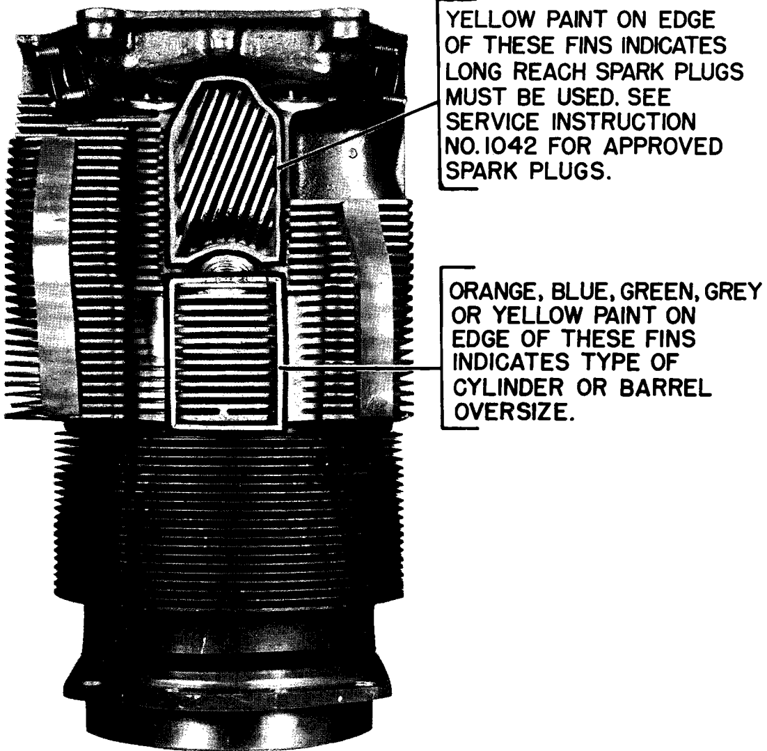
Cylinder Assembly Showing Color Coded Areas
